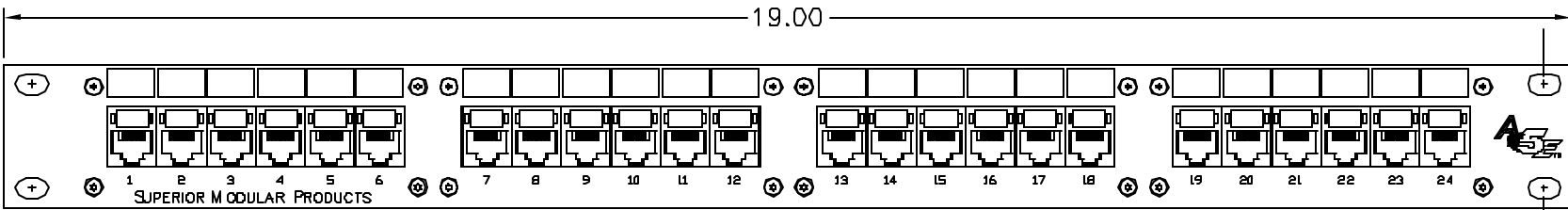
FRONT VIEW
